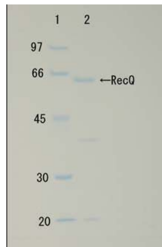
Fig. 1 : Polyacrylamide gel electrophoresis of RecQ protein.
